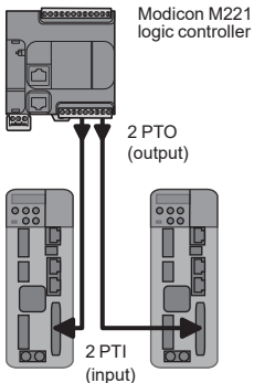
Example of architecture with two LXM28A servo drives controlled by Modicon M221 logic controller
