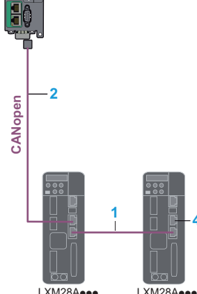
Examples of architectures with control by Modicon M241/M251 logic controllers or LMC058 motion controller
